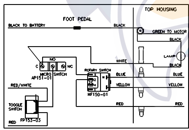
12/24 WIRING DIAGRAM
